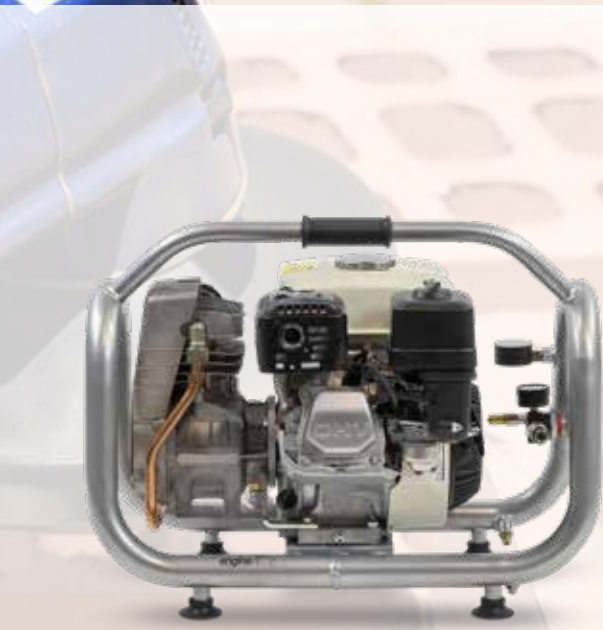
engineAIR 5/2,5 10 PETROL
